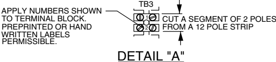
DETAIL "A"
